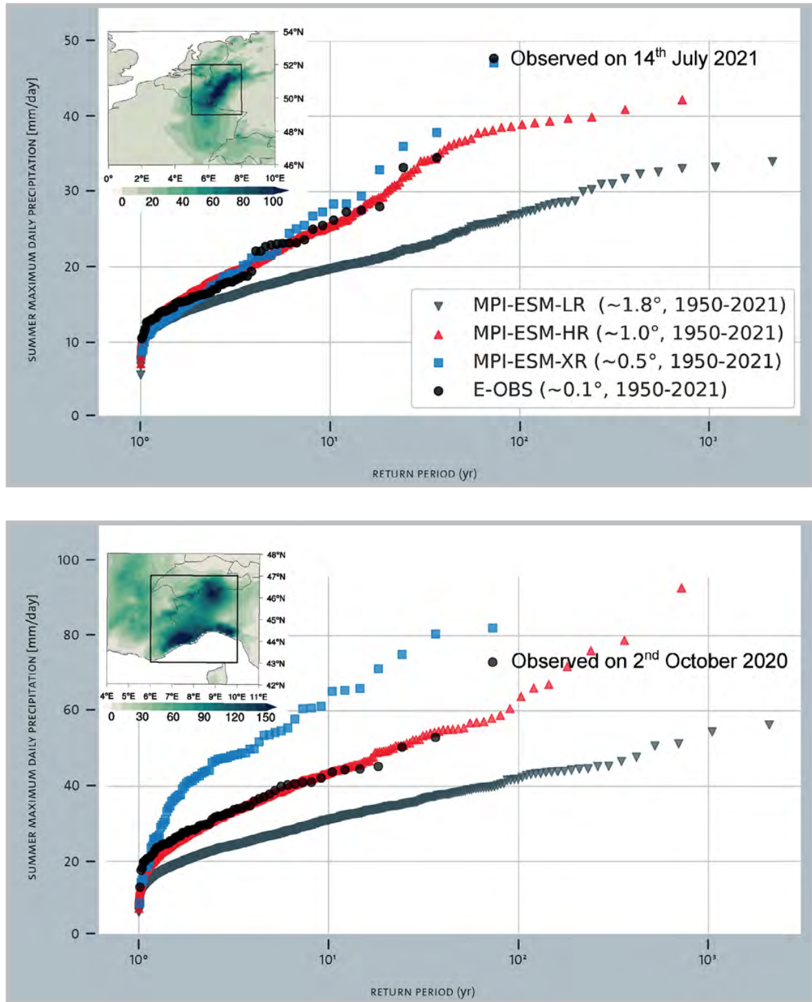
Figure 4.2: Representation of observed heavy precipitation extremes dependent on model spatial resolution: Return periods of (upper panel) summer (JJA) maximum daily precipitation averaged across the western European box, and (lower panel) autumn (SON) maximum daily precipitation averaged across the Western Alps box from 1950-2021 in three model resolutions from MPI-ESM1.2 and in observations. MPI-ESM-LR is based on 30, MPI-ESM-HR on 10, and MPI-ESM-XR and the E-OBS observations on only a single realization. Values of all summers or autumns and all realizations are merged for each ensemble (adapted from Olonscheck et al., 2023).
